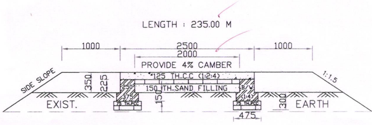
X-SECTION OF ROAD
